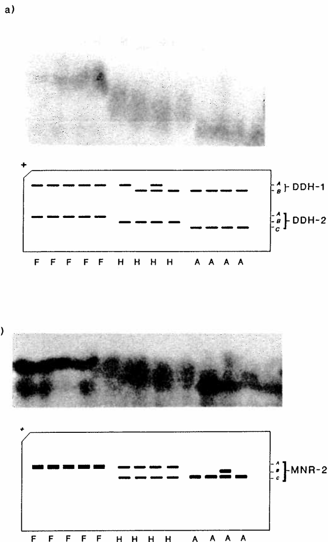
Figure 2 Zymograms showing (a) the alternative (DDH-1) and intermediate (DDH-2) positions of allele mobilities, and (b) shared mobilities at MNR-2 for the A. arborescens × A. ferox hybrids using histidine-citrate buffers with pH of 5.7 and 6.5 respectively (F = A. ferox , H = hybrid, A = A. arborescens ).
