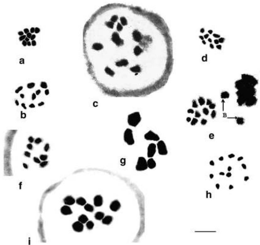
Fig. 1. Microphotographs of meiotic chromosomes of some South African Umbelliferae. (a) Anginon difforme (n=11); (b) A. paniculatum (n=11); (c) A. swellendamense (n=11); (d) Annesorhiza macrocarpa (n=11); (e) A. macrocarpa with B-chromosomes (n=11+1B) [a second set of chromosomes that did not separate is visible to the right, with their corresponding B-chromosome]; (f) Dasispermum suffruticosum (n=9); (g) Hermas villosa (n=7); (h) Itasina filifolia (n=12); and (i) Lichtensteinia lacera (n=11). Voucher specimens are listed in Table 2. Scale bar=10 \mu m.
